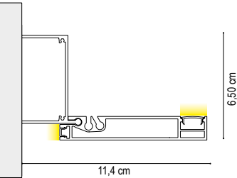
FLOAT L LED MONOCOLORE
