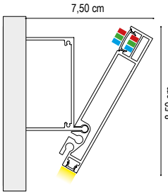
FLOAT K LED MONOCOLORE + RGB
