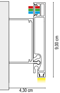
FLOAT I LED MONOCOLORE + RGB
