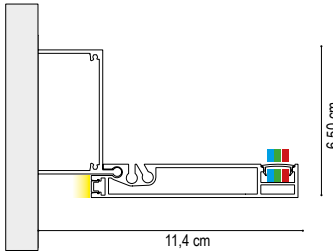
FLOAT L LED MONOCOLORE + RGB
