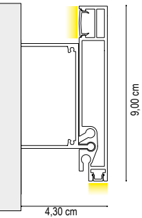
FLOAT I LED MONOCOLORE
